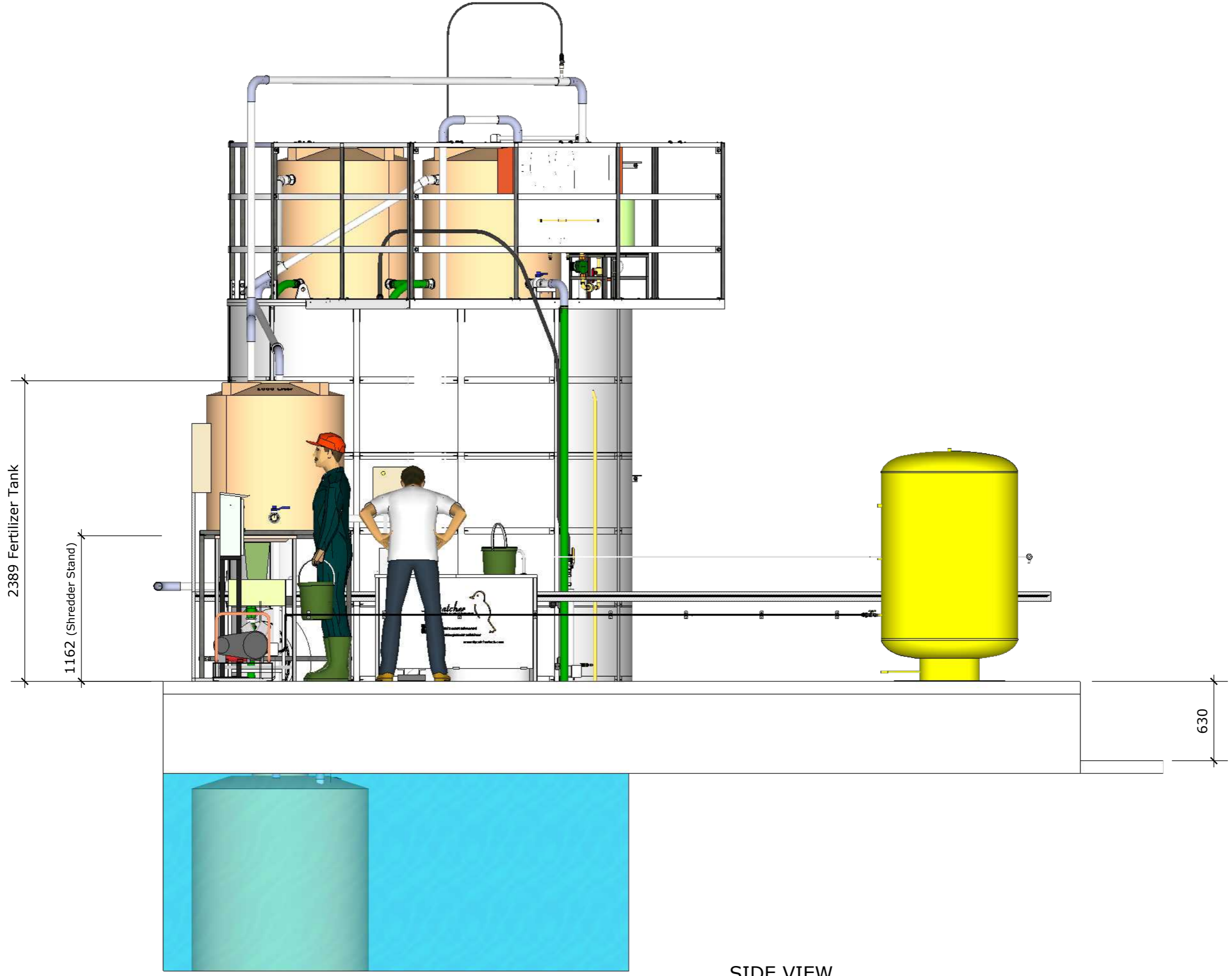
SIDE VIEW
