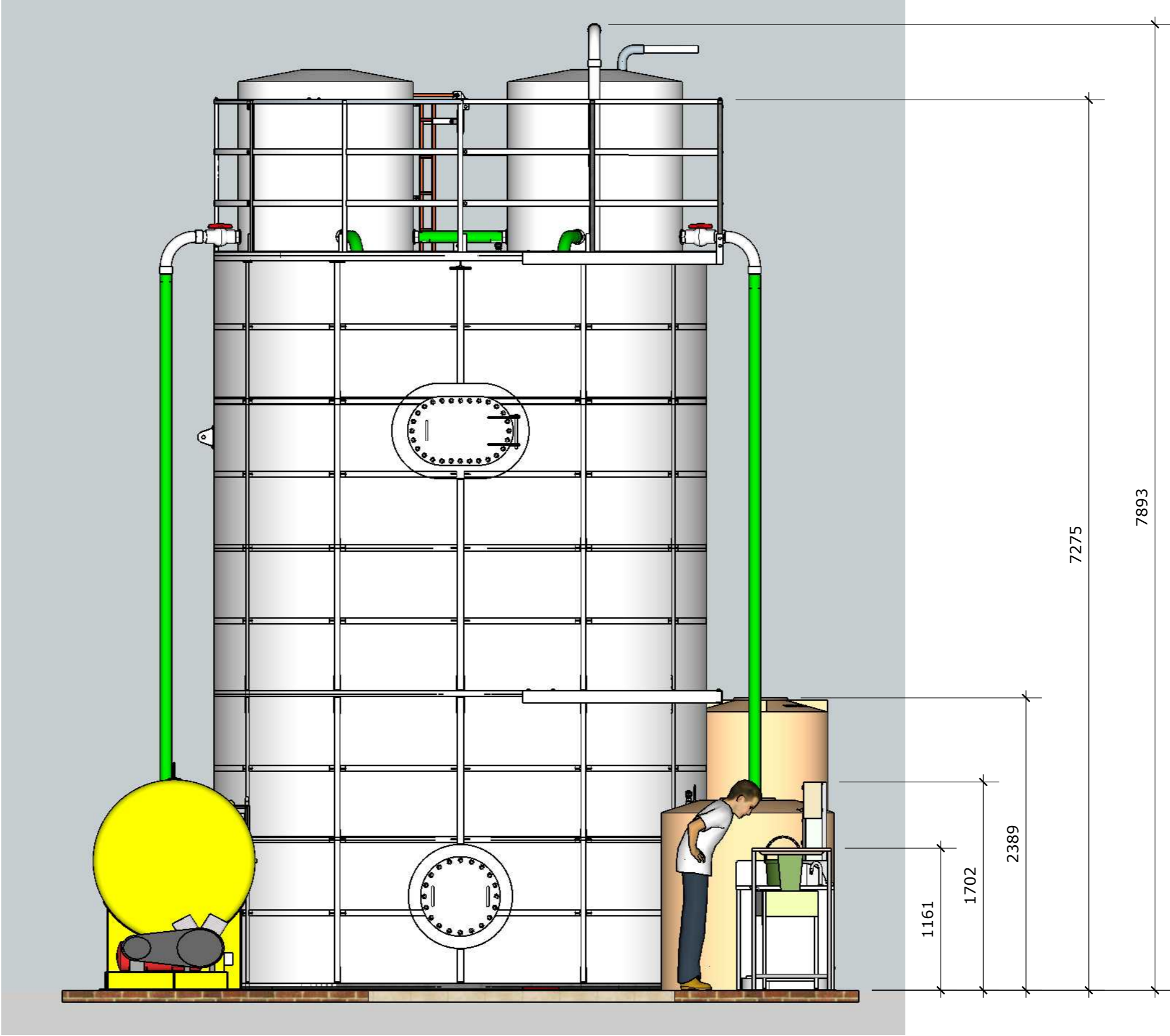
SIDE VIEW
