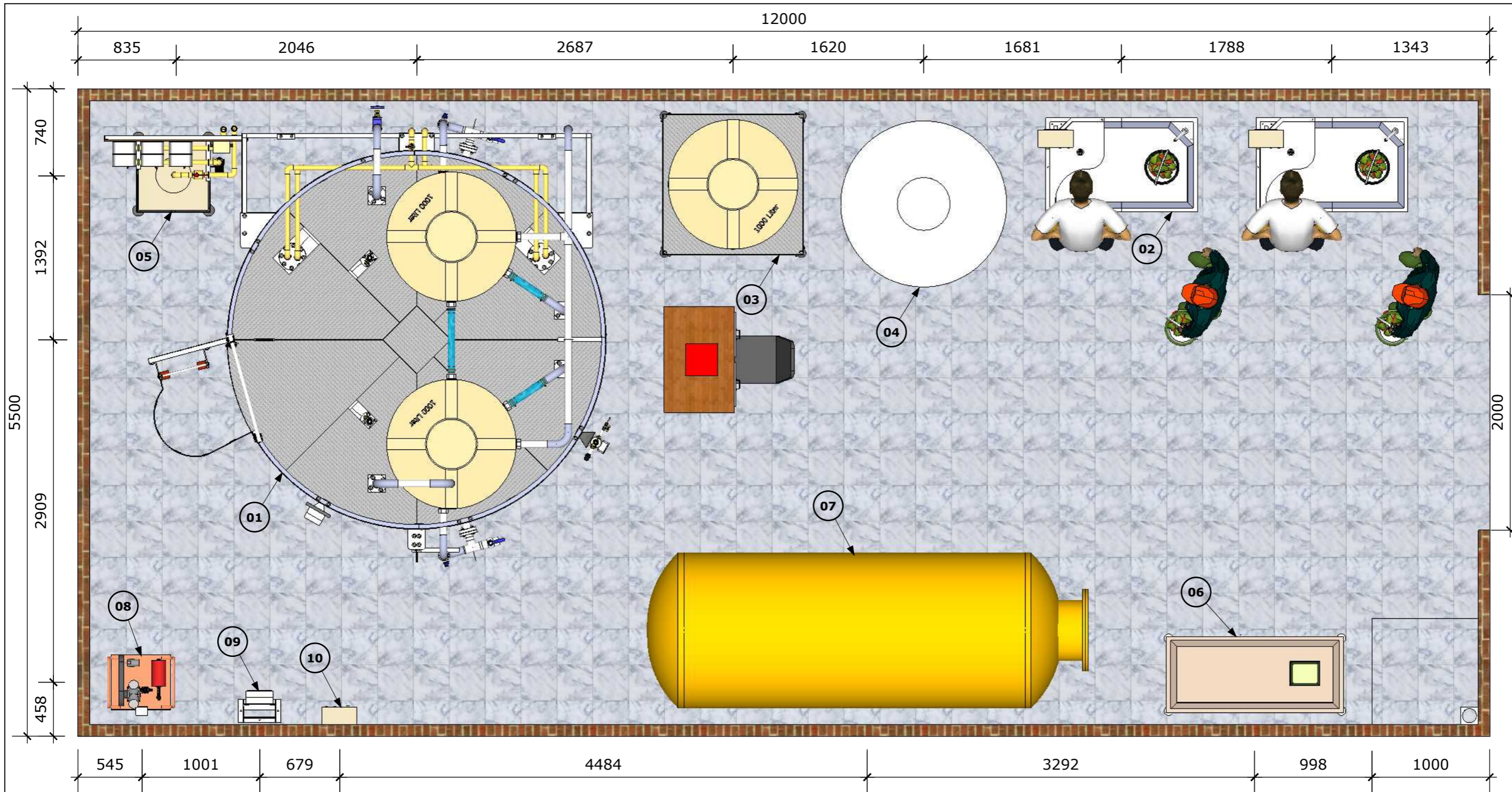
PLAN VIEW
