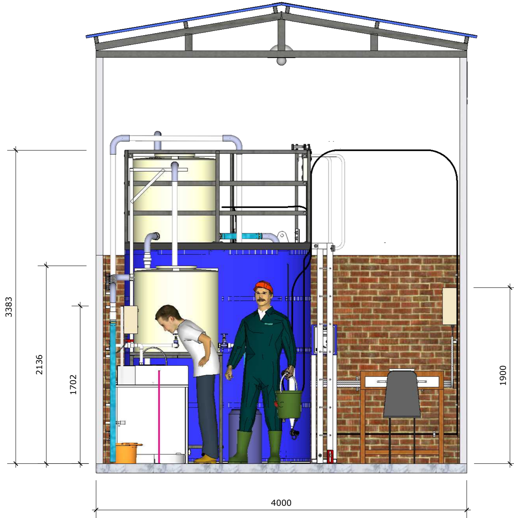
SIDE VIEW
